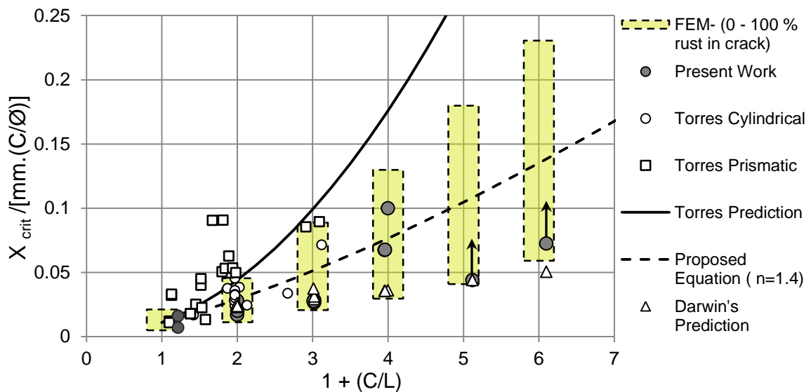
Figure 5.22 Comparison of FE model findings (for \alpha=3 and d_o=20 \mu m ) with current and previous experimental results and existing model predictions with partially corroded cases treated as per approach 2. The bottom and top ends of the yellow floating bars represent zero and 100% rust in crack, respectively. The symbols shown with arrows indicate un-cracked specimens.
