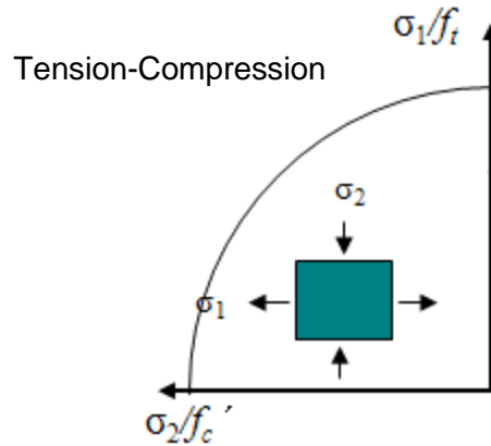
Figure 5.5 Cracking failure envelope in Tension-Compression domain [Luc 2010]
