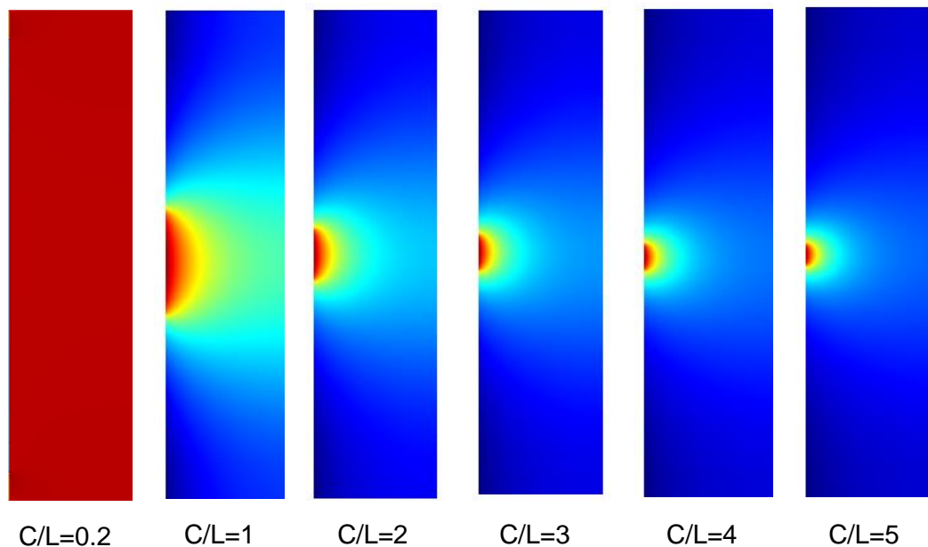
Figure B.16 Potential distribution trends across concrete cover for the localized corrosion cases considering the 100% macrocell current scenario and for the uniform corrosion case. (Potential levels were reported in chapter 5)
