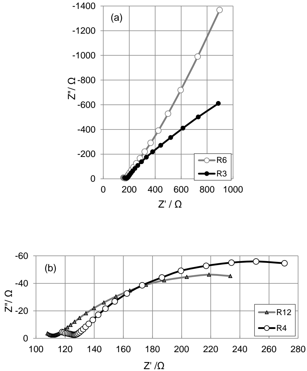
Figure 4.5 EIS integrated response over the entire embedded steel surface (400 mm 2 ) for pre-cracked specimens having nominal crack widths: (a) 0.5 mm and (b) 2.5 mm after 95 days of continuous chloride ponding. Frequency range 1 mHz to 1000 Hz, 5 points / decade.
